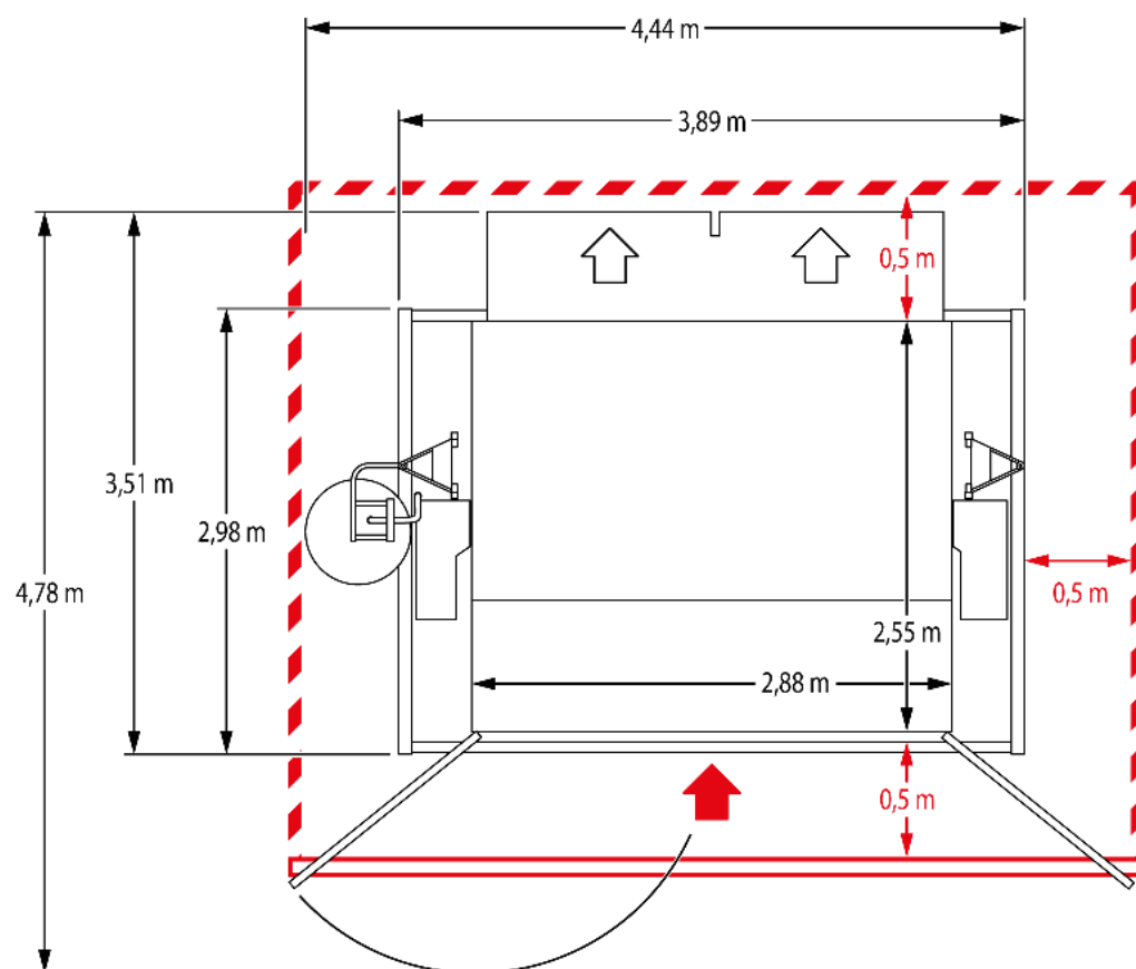
III. 23: Espace requis plateforme ED+
