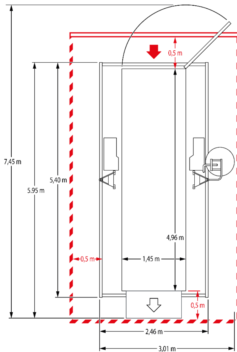
III. 11: Espace requis plateforme BLL
